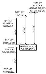
LEFT ELEVATION
